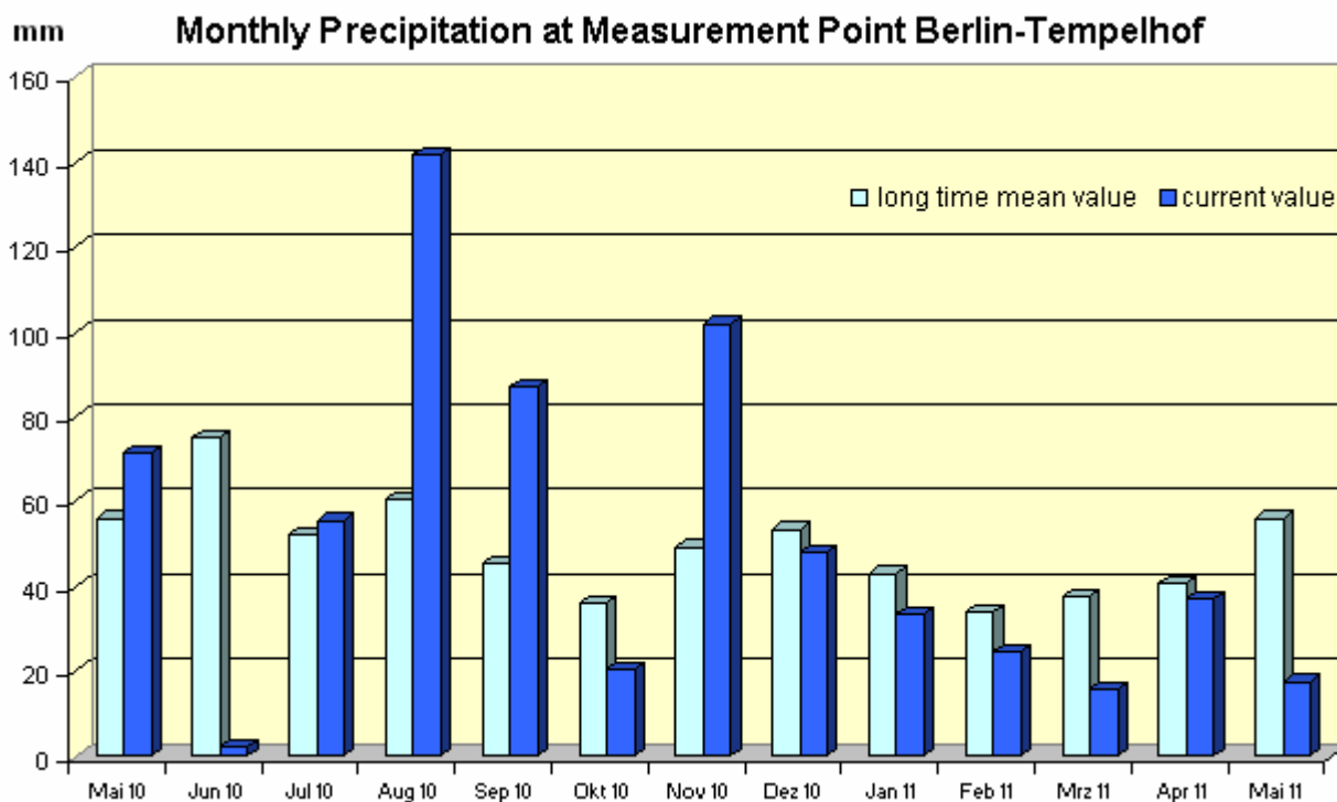
Fig. 14: Monthly precipitation between May 2010 and May 2011 at the Berlin-Tempelhof Measurement Point, compared with the long-term mean, 1961 through 1990.
