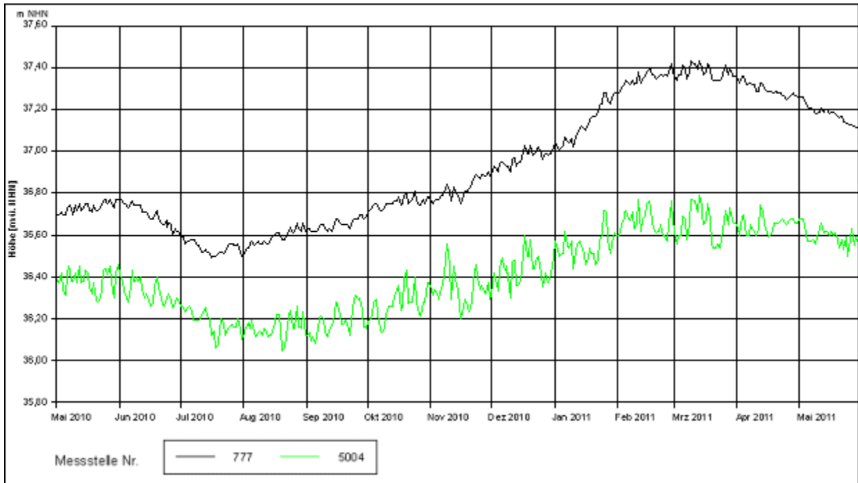
Abb. 13: Groundwater level at two measurement points in an exemplary manner on the plateaus on May 2010 to May 2011
