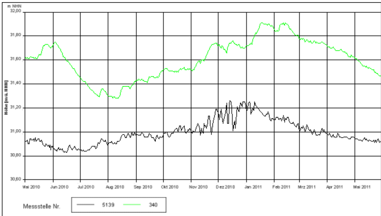
Fig. 12: The groundwater levels at two measurement stations in the glacial spillway on May 2010 to May 2011
