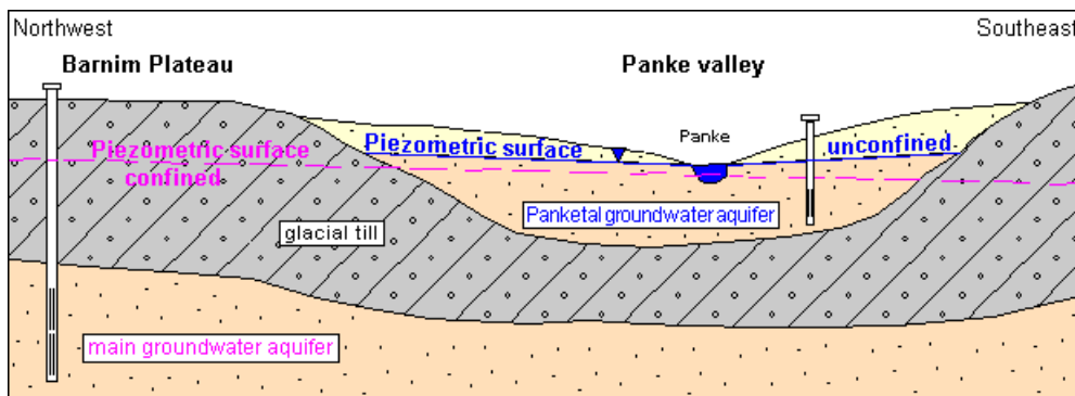
Fig. 7: The Panke Valley aquifer (aquifer 1) is situated above the main aquifer (aquifer 2) separated by the clay-layer of the ground moraine.
