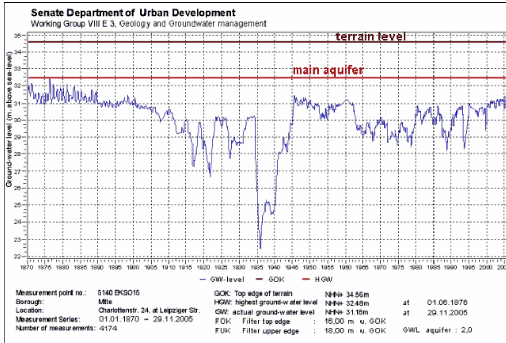
Fig. 8: Hydrographic Curve of Groundwater Levels at a Measurement Point in the Borough of Mitte, from 1870 to the Present
