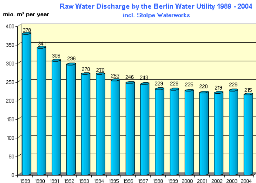
Fig. 9: Drop in Raw-Water Discharge by the Berlin Water Utility during the Past 15 Years
