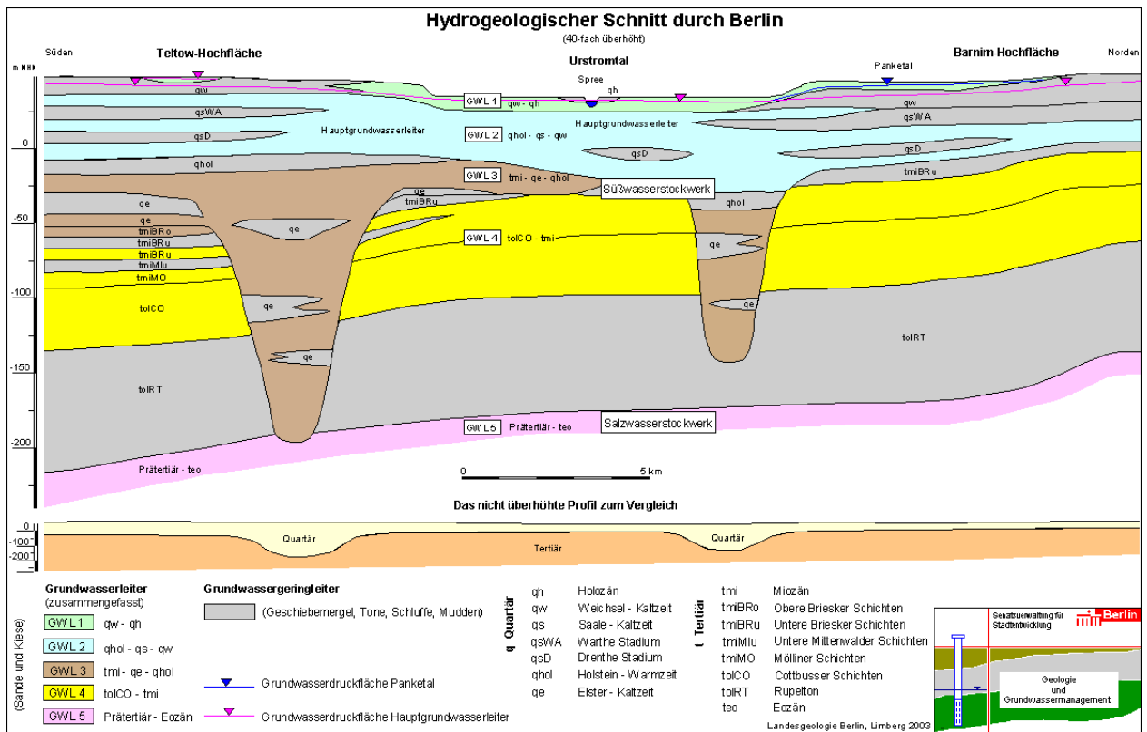
Fig. 6: Hydrogeological Cross-Section of Berlin
