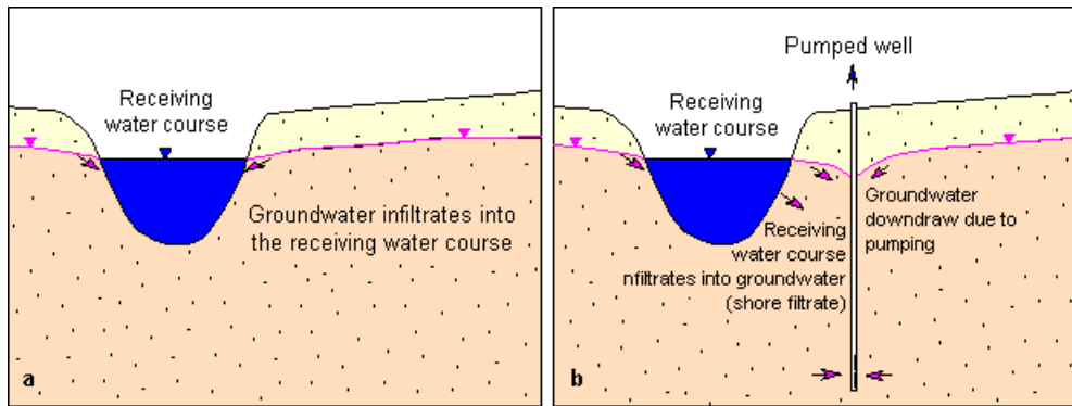
Fig. 4: Infiltration: a) Effluent condition (left), b) Influent condition (right)
