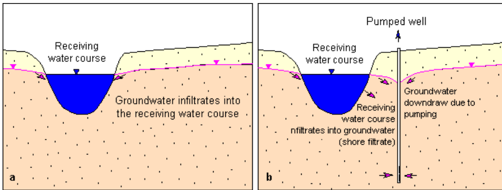
Fig. 4: Infiltration: a) Effluent condition, b) Influent condition
