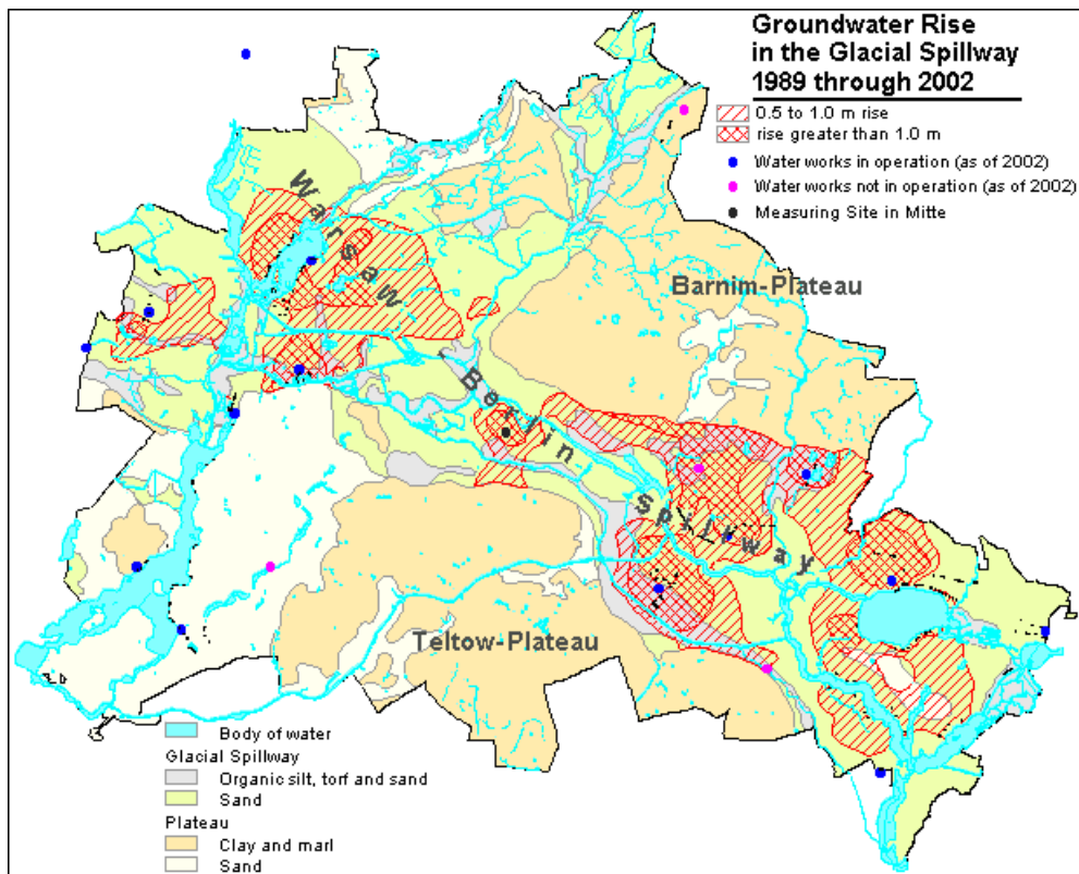
Fig. 10: Groundwater Rise in the Glacial Spillway between 1989 and 2002. (to Hydrographic Curve of Groundwater Levels at a Measurement Point in the Borough of Mitte, from 1870 to the Present, s.a. Fig. 8)
