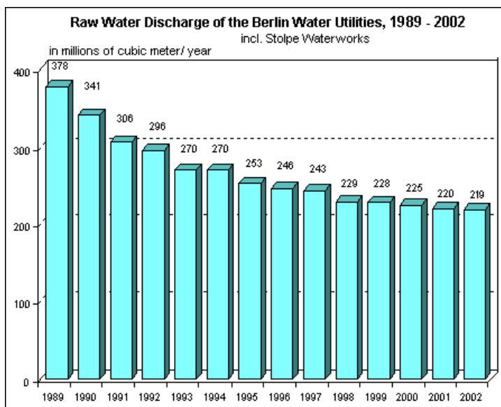
Fig. 9: Drop in Raw-Water Discharge by the Berlin Water Utility during the Past 14 Years
