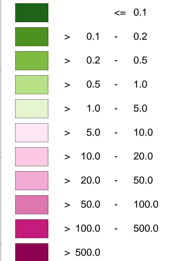
Emissions of domestic fuel 2005 (t/km² a)
