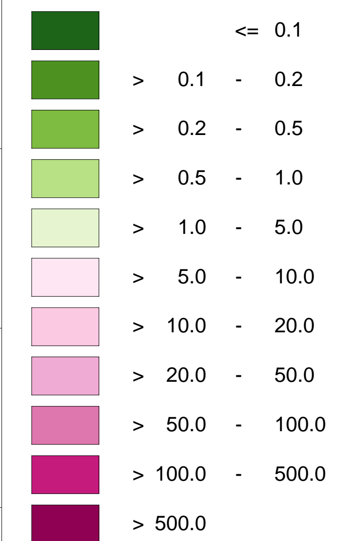
Emissions of domestic fuel 1994 (t/km² a)
