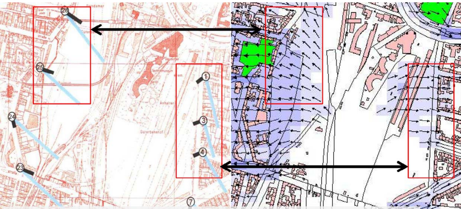
Climate simulation 2009 (spatial resolution 50m*50m)
