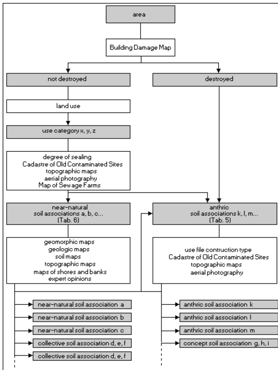
Fig. 1: Classification of Soil Associations, Schematic Depiction of Procedure
