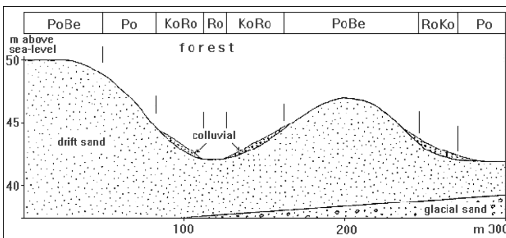
Fig. 4: Spodo-dystric Cambisol (podzol-brown soils) - Podzols - Colluvial Dystic Cambisols (colluvial rusty brown soil) (soil association of dunes of fine sand)
