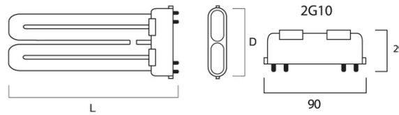
TECHNICAL DRAWINGS
